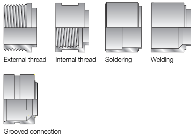
Grooved connection
