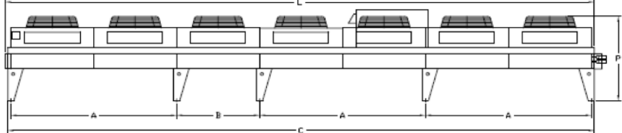
FRONT VIEW FEVK17
