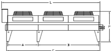
FRONT VIEW FEVK14 & FEVK24
