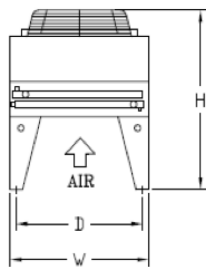
END VIEW FEV*11
