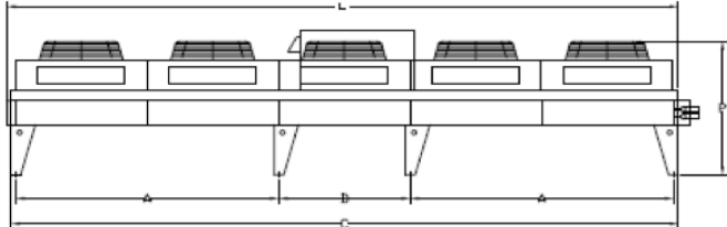
FRONT VIEW FEVK16
