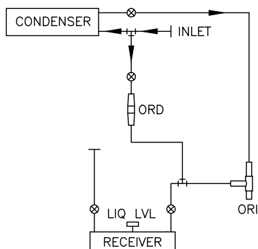
RECEIVER PIPING
